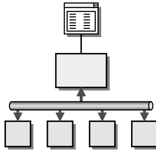
Service-Oriented Architecture
