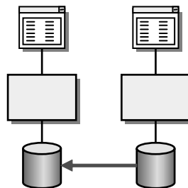
Data Replication
