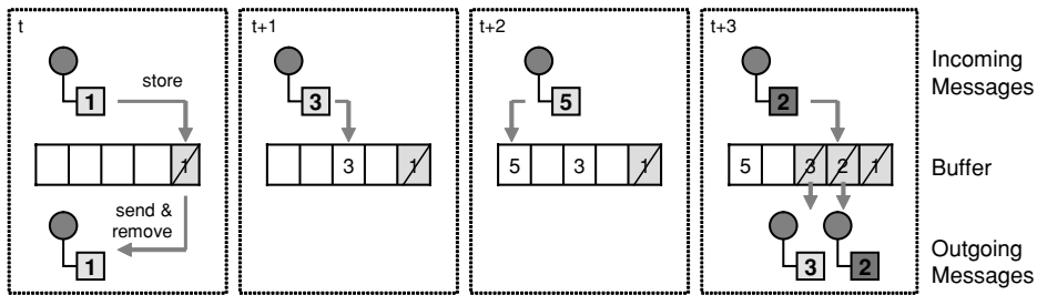
Internal Operation of the Resequencer
