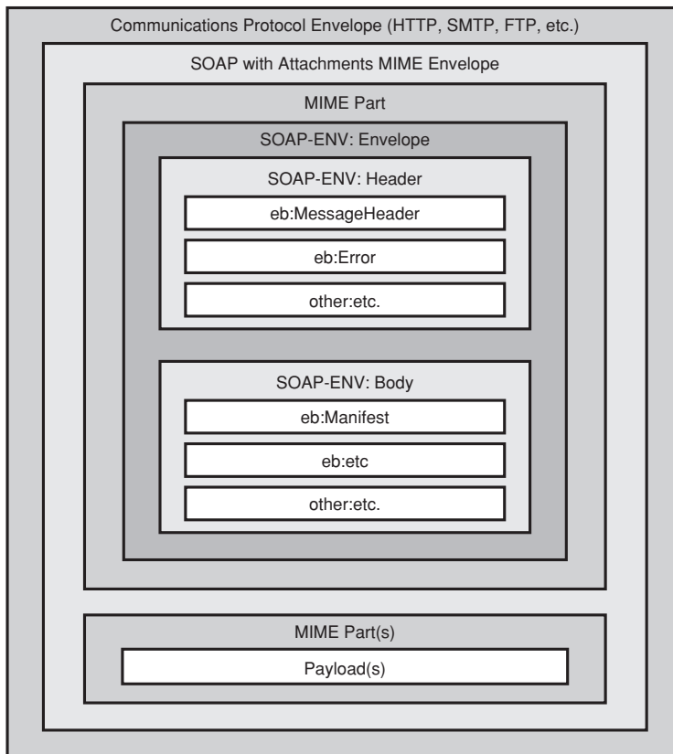
An ebMS Message Is Composed as SOAP Messages with Attachments
