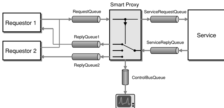
Simple Smart Proxy Example
