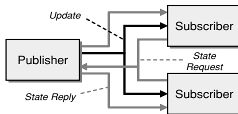
Publish-Subscribe Using the Pull Model
