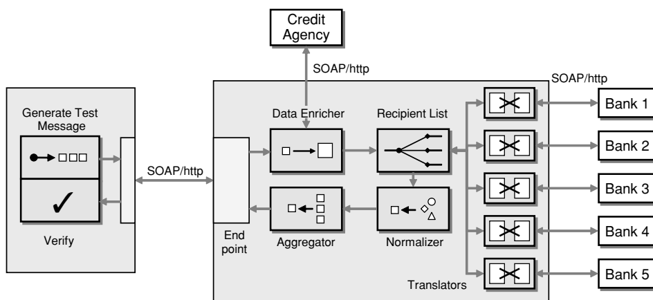
Web Services Solution Architecture
