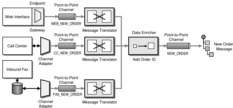
Taking Orders with Enricher
