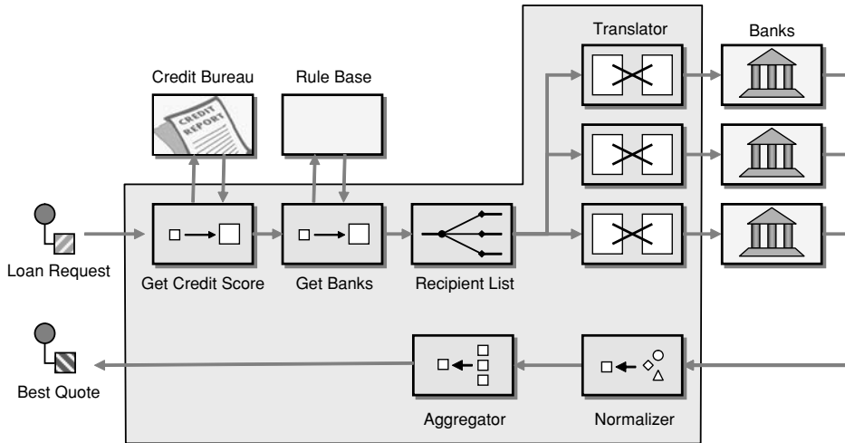
Complete Loan Broker Design
