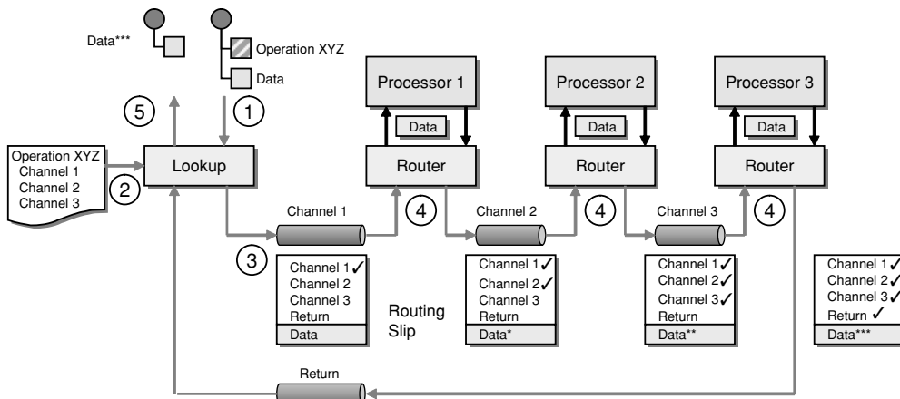
Using a Routing Slip as a Composed Service
