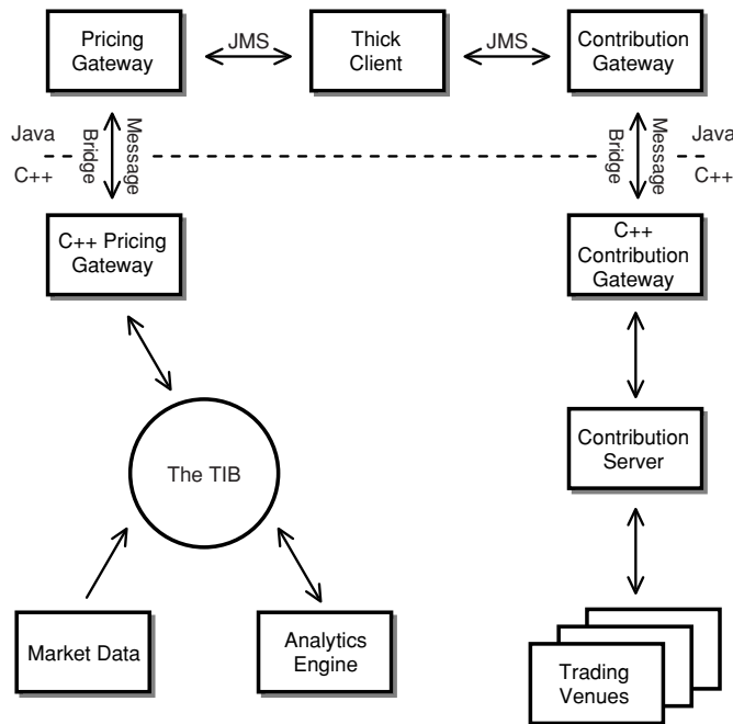
The Current System with the Channel Adapters
