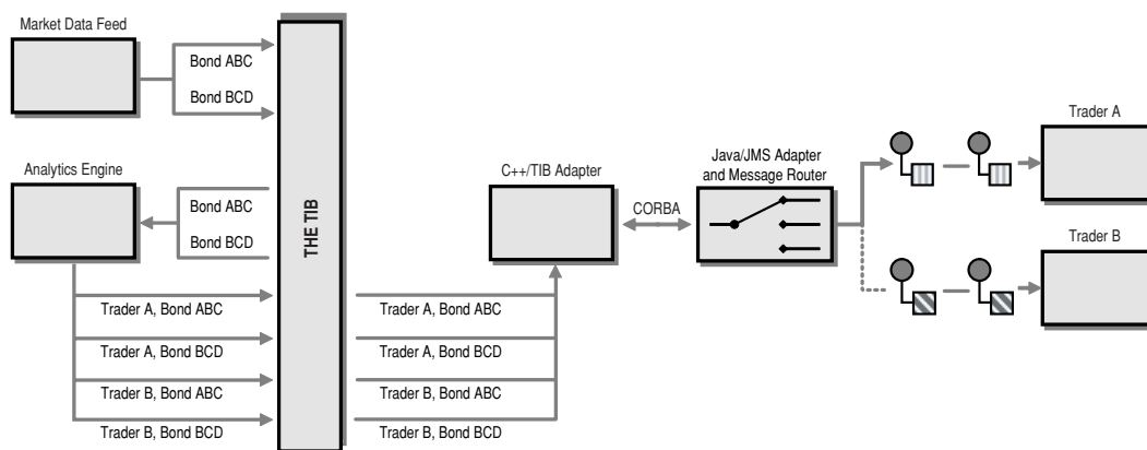
The Complete Market Data Flow to the Client
