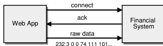
Tightly Coupled Interaction
