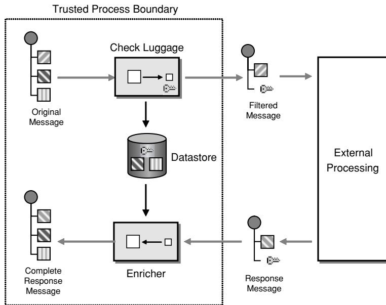
Eliminating Sensitive Message Data Outside of the Trusted Process Boundary
