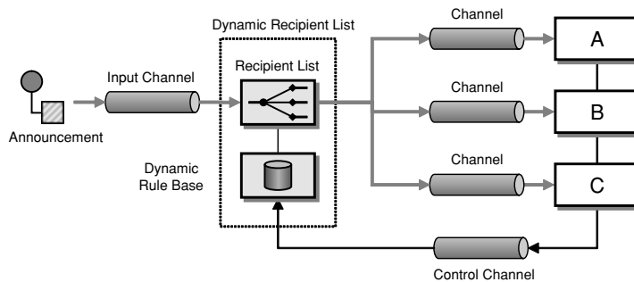
Sending Announcements with a Dynamic Recipient List
