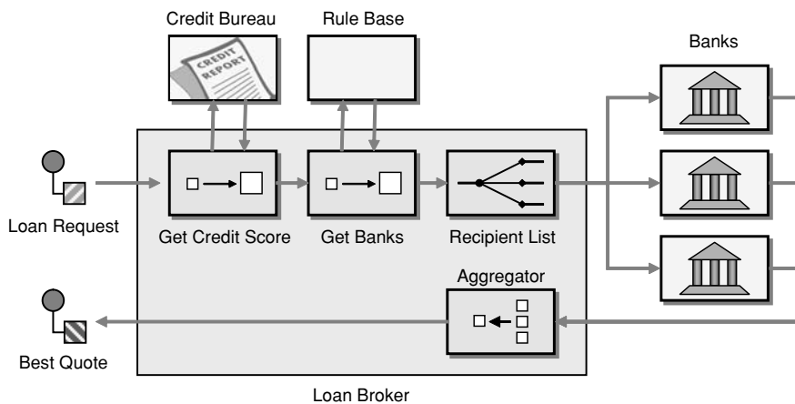
Simple Loan Broker Design
