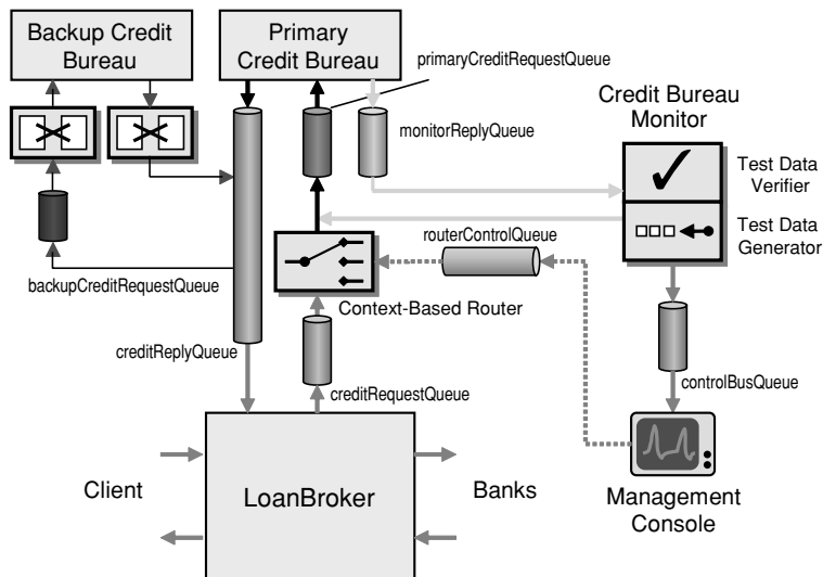
Explicit Failover with a Context-Based Message Router
