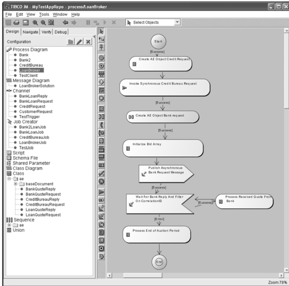
The Loan Broker Process Definition
