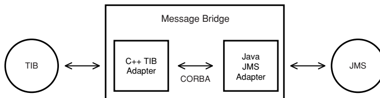
Messaging Bridge Using Channel Adapters
