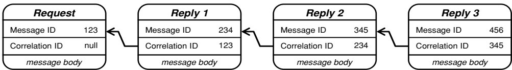
Request-Reply Chaining
